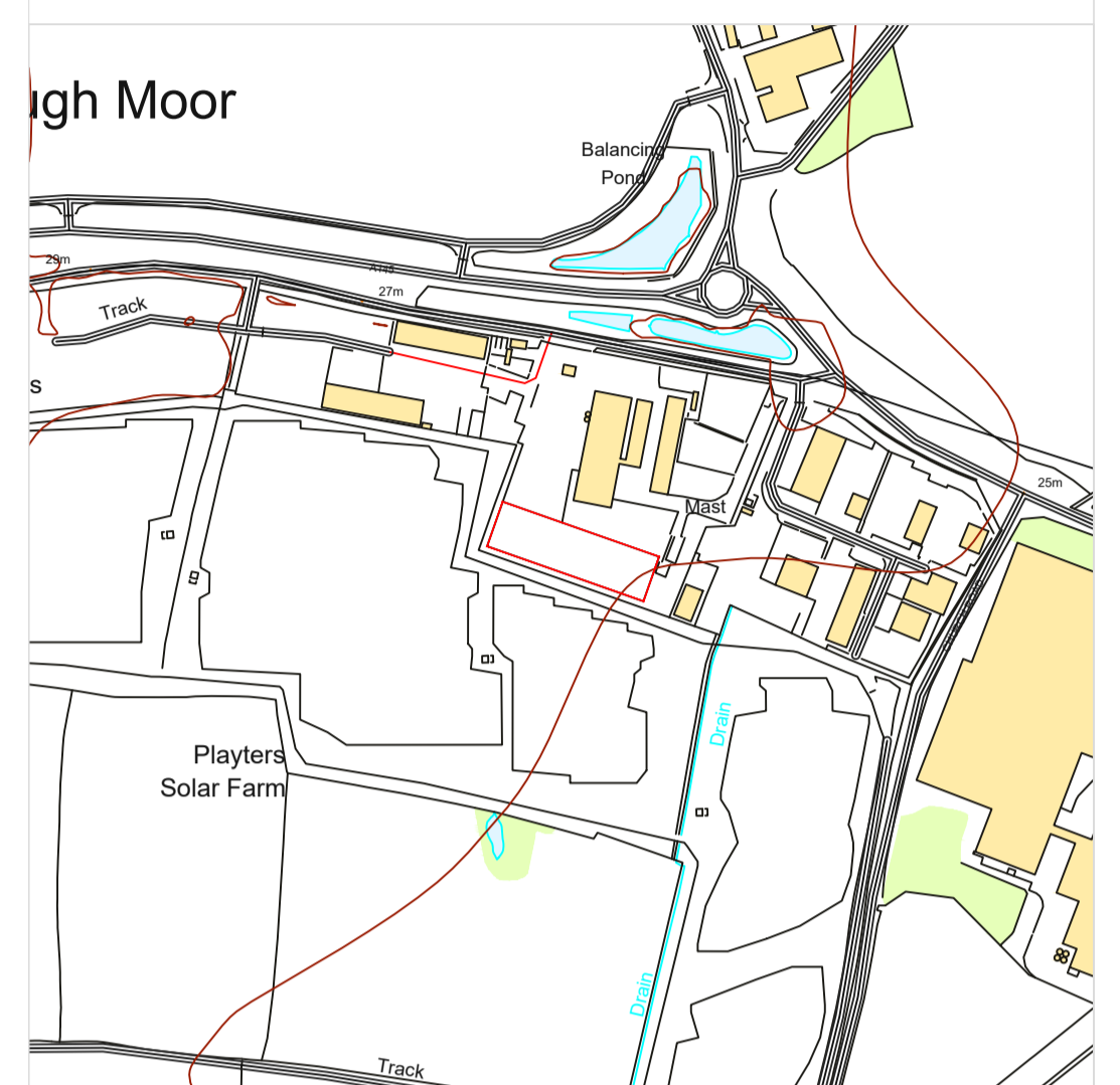
LOCATION PLAN 1:5000
